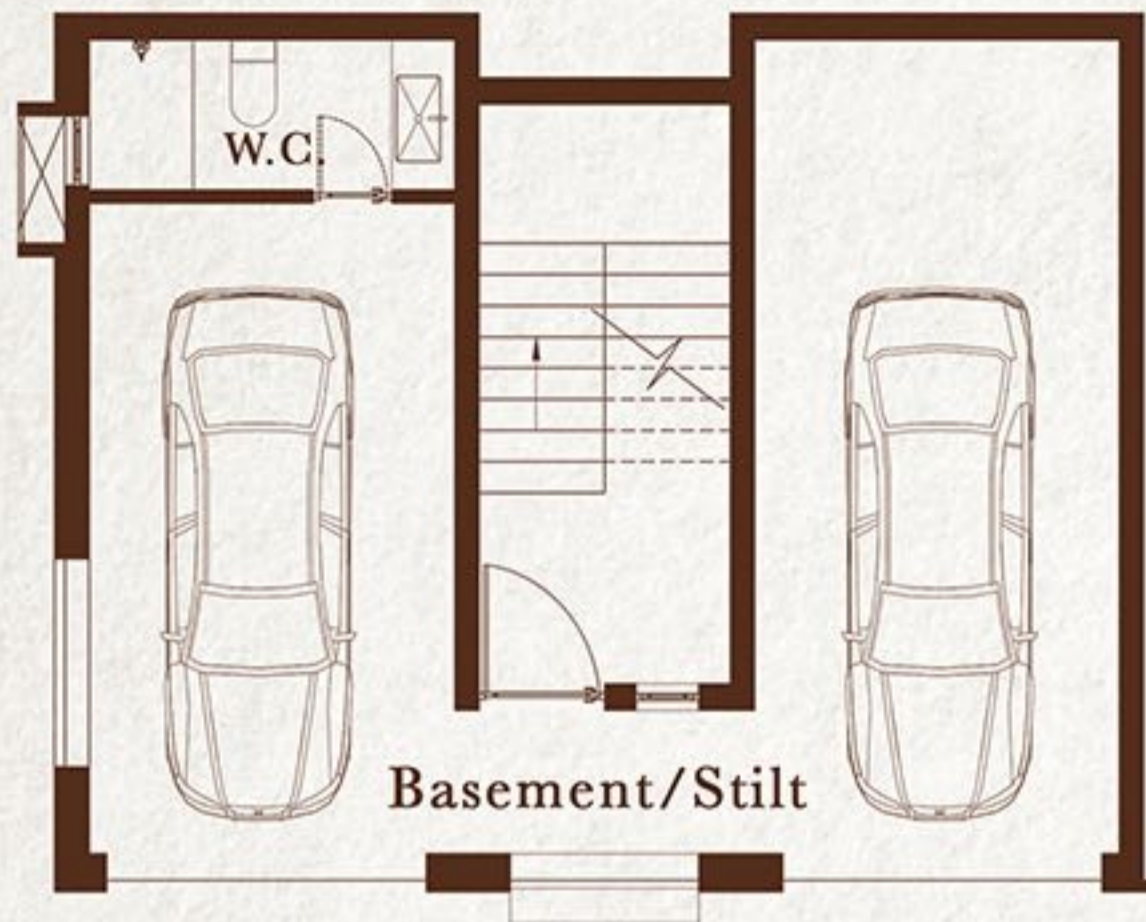
BASEMENT/STILT LEVEL PLAN
